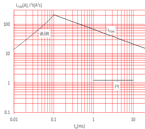
FIG.5: Non-repetitive surge peak on-state current for a sinusoidal pulse with width t_p < 20ms , and corresponding value of I^2t ( di/dt < 60A/\mu s )
