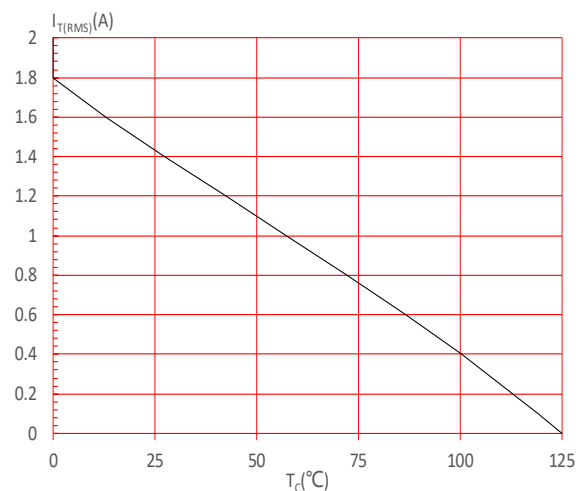
FIG.4: On-state characteristics
