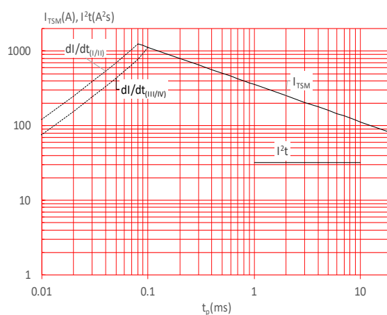
FIG.6: Non-repetitive surge peak on-state current for a sinusoidal pulse with width t_p < 20ms , and corresponding value of I^2t ( I - II : dl/dt < 100A/\mu s ; III-IV : dl/dt < 50A/\mu s )
