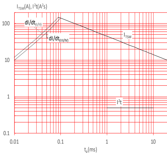
FIG.5: Non-repetitive surge peak on-state current for a sinusoidal pulse with width t_p < 20\text{ms} , and corresponding value of I^2t (I - II : di/dt < 50\text{A}/\mu\text{s} ; III-IV : di/dt < 30\text{A}/\mu\text{s} )
