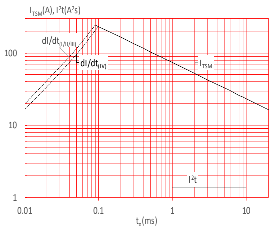
FIG.5: Non-repetitive surge peak on-state current for a sinusoidal pulse with width t_p < 20ms , and corresponding value of I^2t (I - II - III: di/dt < 70A/\mu s ; IV: di/dt < 40A/\mu s )
