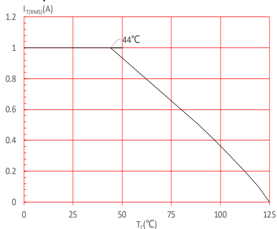
FIG.4: On-state characteristics
