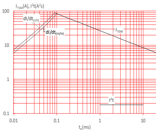
FIG.5: Non-repetitive surge peak on-state current for a sinusoidal pulse with width t_p < 20\text{ms} , and corresponding value of I^2t ( I - II: di/dt < 50\text{A}/\mu\text{s}; III - IV: di/dt < 20\text{A}/\mu\text{s} )
