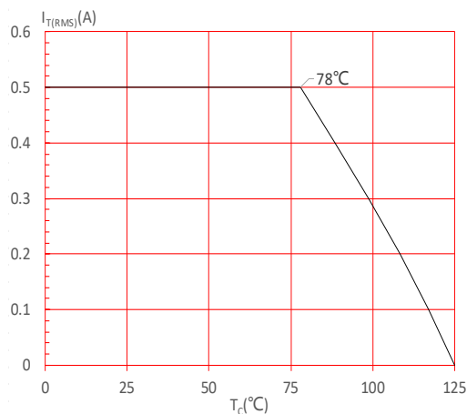
FIG.4: On-state characteristics
