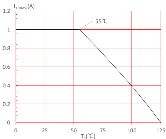
FIG.4: On-state characteristics
