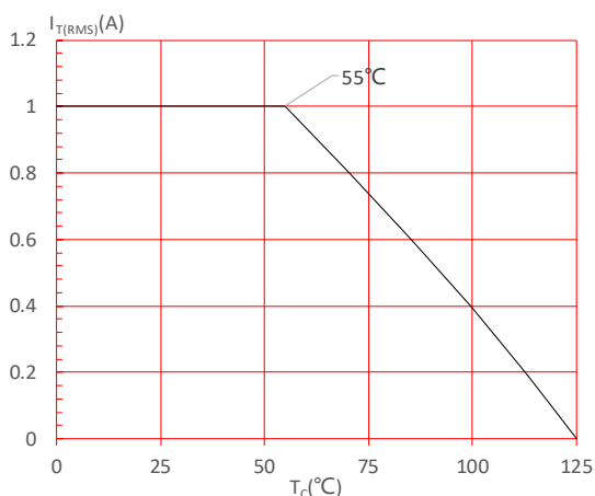
FIG.4: On-state characteristics
