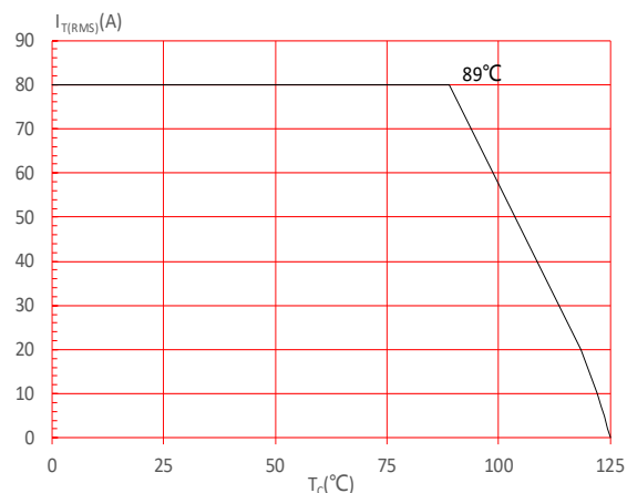
FIG.4: On-state characteristic
